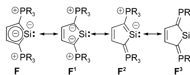
Scheme 2. Resonance structures of the carbocyclic ylide-stabilized silylene F .
